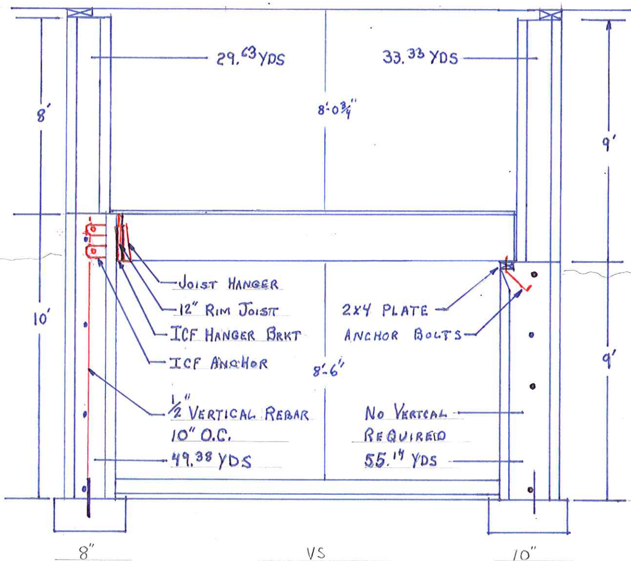
EXAMPLE USING 200 LINFIT OF WALL WITH 9' OF BACKFILL
